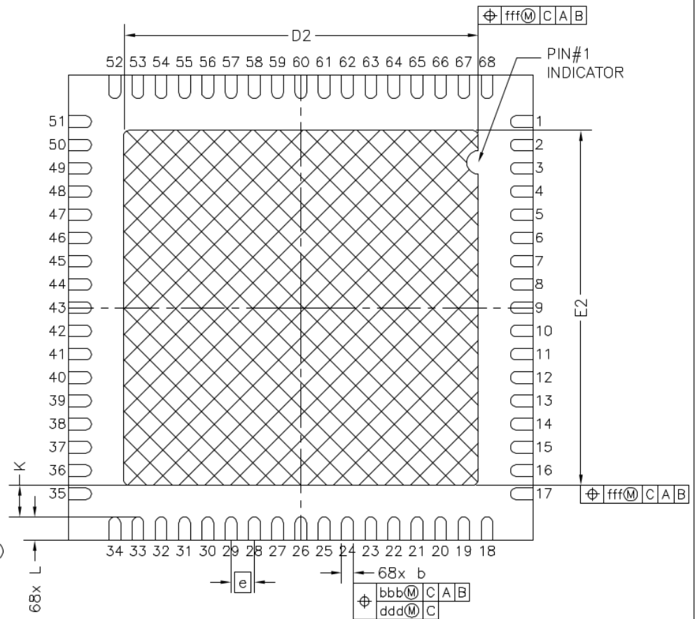
BOTTOM VIEW
