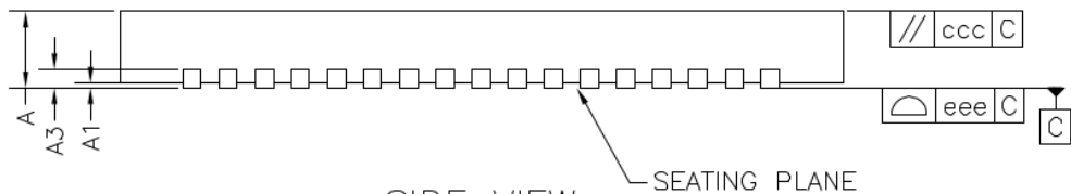
SIDE VIEW
