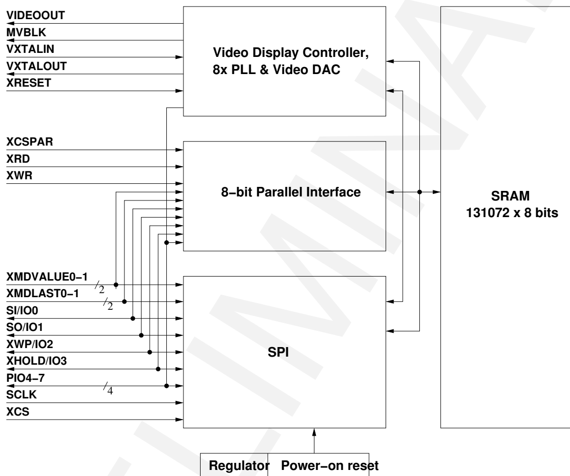
Figure 14: Device Organization
