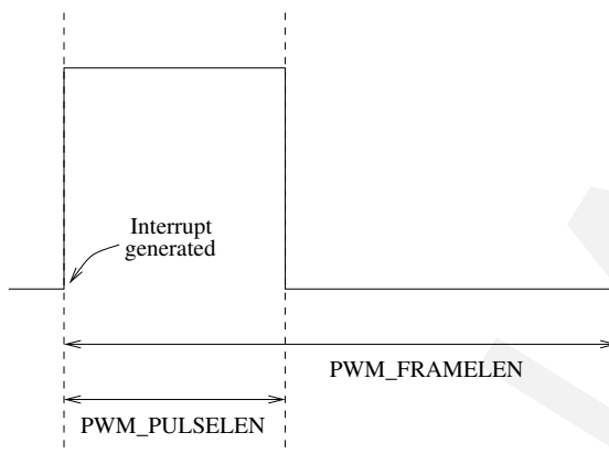
Figure 33: PWM Unit timing diagram
