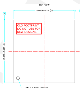
Figure 14: VS1005g top view, OBSOLETE1 LFGA-88
