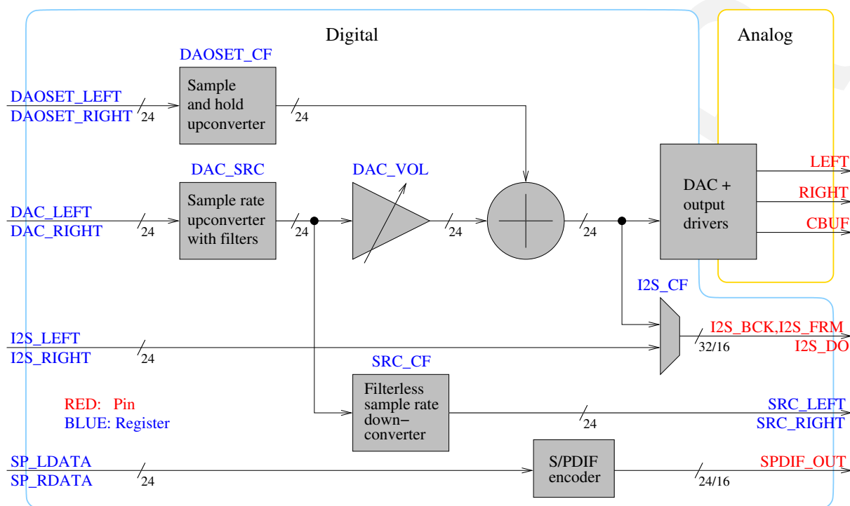
Figure 22: VS1005g playback (DA) audio paths
