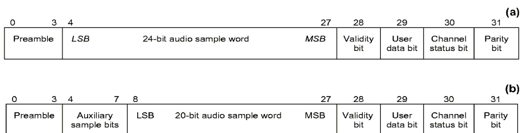
Figure 30: S/PDIF sub-frame format
