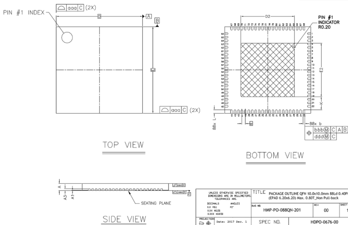
Figure 4: VS1005g QFN-88 mechanical drawing, page 1/2
