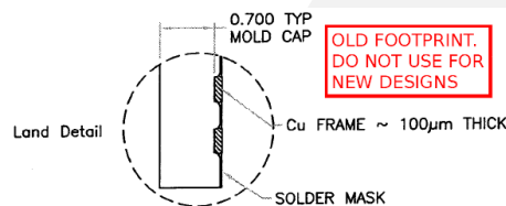
Figure 10: VS1005g corner view, OBSOLETE2 LFGA-88
