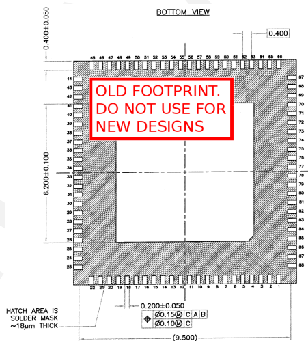
Figure 11: VS1005g bottom view, OBSOLETE2 LFGA-88
