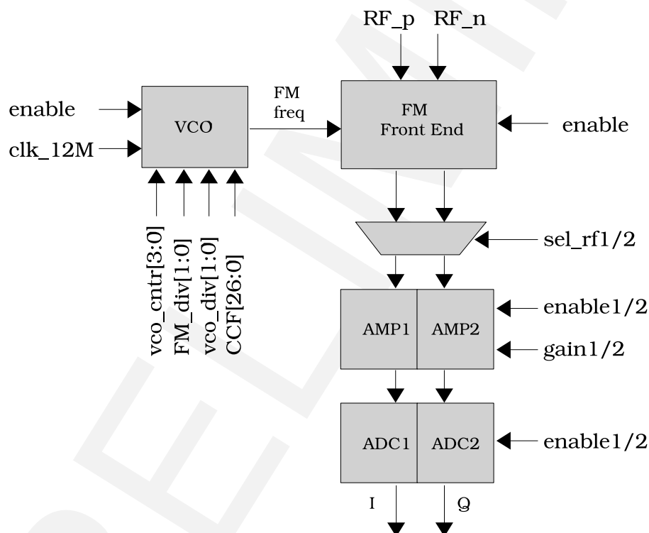
Figure 24: Block diagram of FM receiver, RF and analog section
