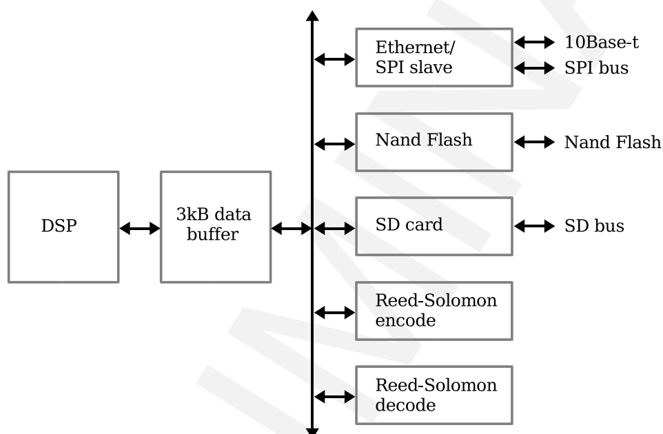
Figure 26: Block diagram of data interfaces
