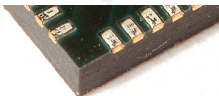
Figure 8: VS1005g OBSOLETE2 LFGA-88 bottom corner view photo
