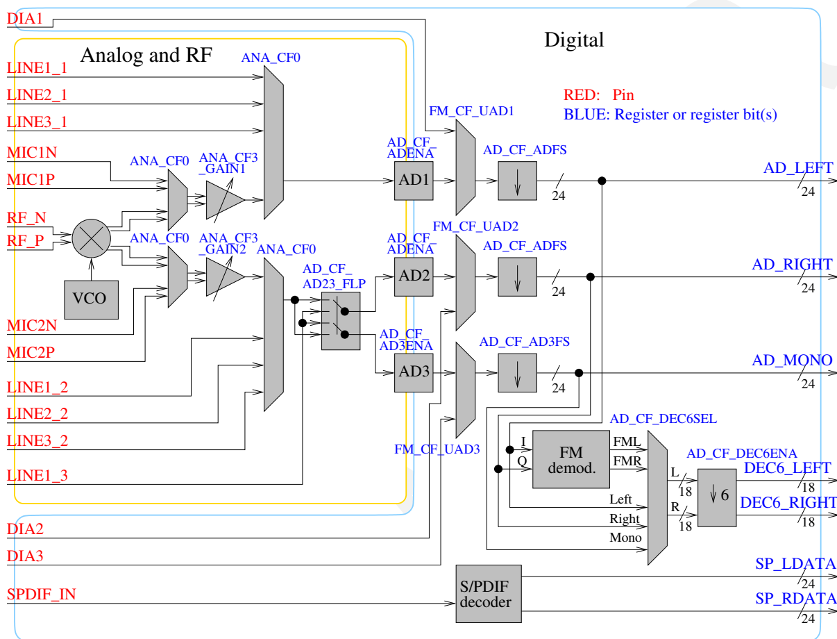
Figure 23: VS1005g recording (AD and FM) signal paths
