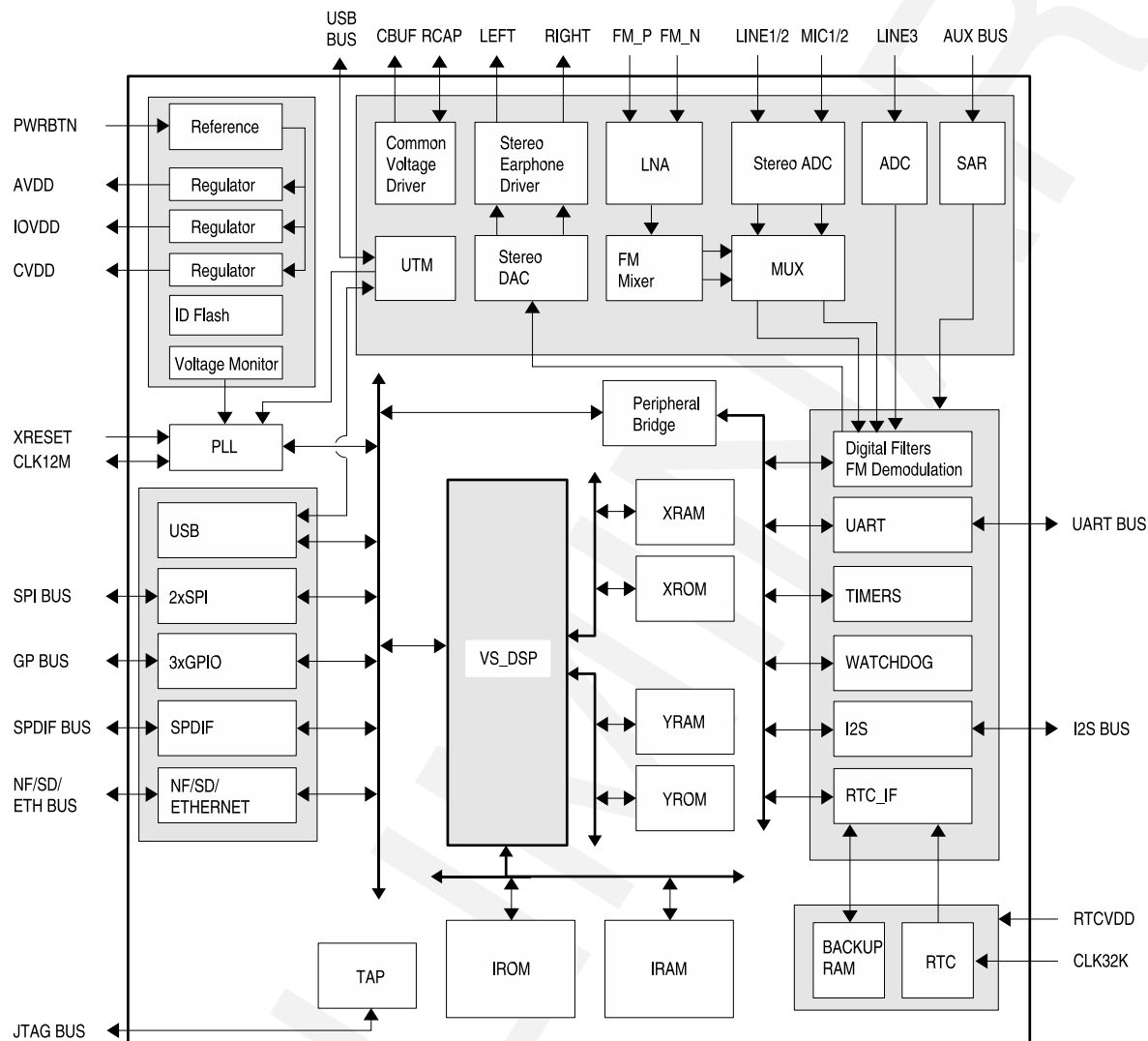
Figure 20: VS1005g block diagram
