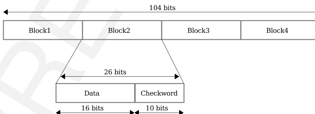
Figure 25: Structure of the RDS baseband coding group
