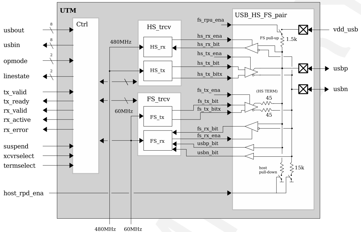
Figure 28: VS1005g UTM functional block diagram
