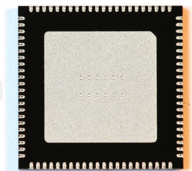
Figure 2: VS1005g QFN-88 bottom view photo, pin 1 top right
