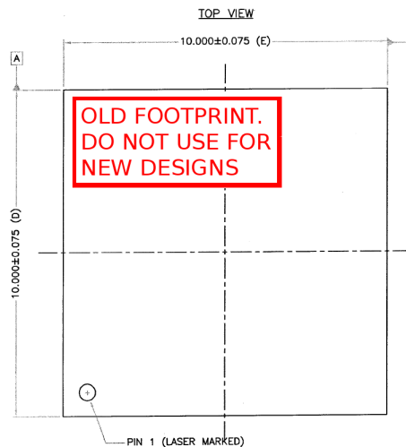
Figure 9: VS1005g top view, OBSOLETE2 LFGA-88
