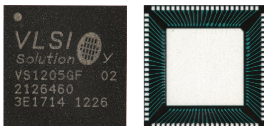
Figure 13: VS1005g OBSOLETE1 LFGA-88 (VS1205G-F product variant) top & bottom photo
