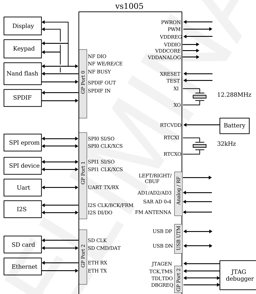
Figure 19: VS1005g external interfaces
