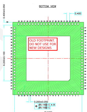
Figure 15: VS1005g bottom view, OBSOLETE1 LFGA-88
