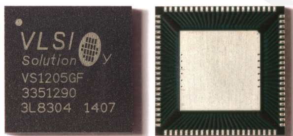
Figure 6: VS1005g OBSOLETE2 LFGA-88 (VS1205G-F product variant) top & bottom photo
